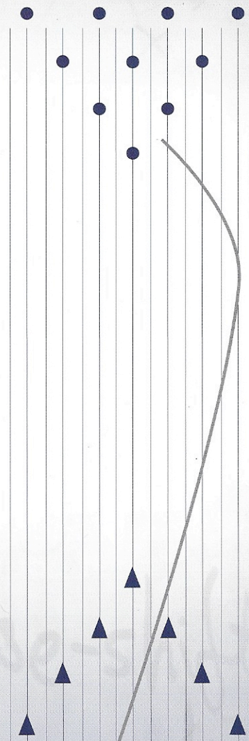
Kinetic Energy
