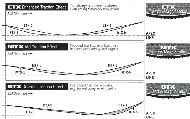
Throbot Traction Comparison Chart
